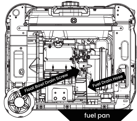
Figure 13: Fuel drain hose
