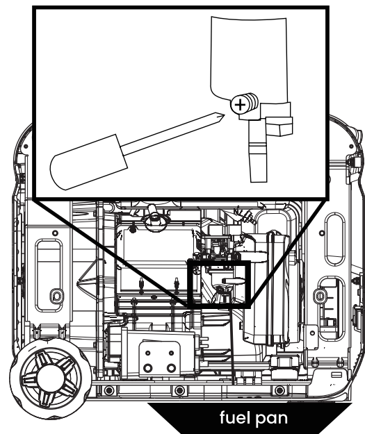
Figure 14: Loosen float bowl screw
