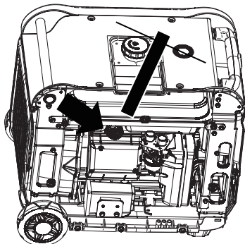
Figure 16: Slide off spark plug cover
