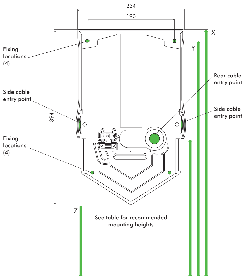
REAR ELEVATION
